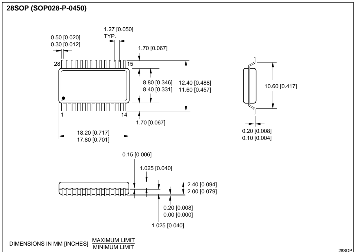
28-pin, 450-mil SOP
